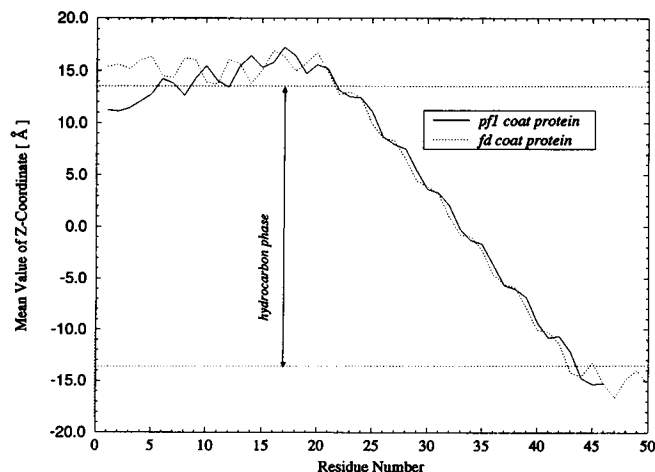
FIGURE 5 Mean (over one simulation cycle) values of the z coordinates of the residues of fd and pf1 coat proteins plotted as a function of residue number. The figure indicates considerable similarity between the structure of pf1 coat protein and the predicted structure of the fd coat protein.
