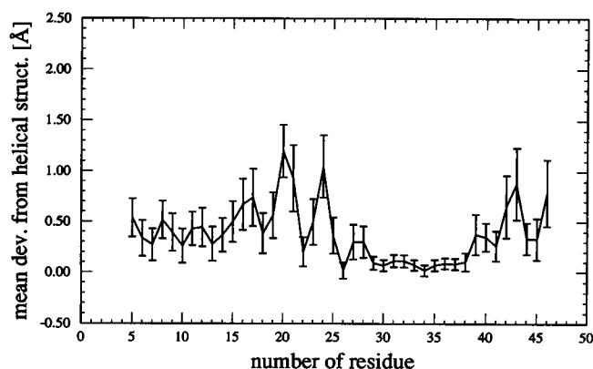
FIGURE 6 The mean (over one simulation cycle) deviations from an "ideal" helix structure for residues in the fd model. The bars denote values of the mean absolute deviation of the data.
